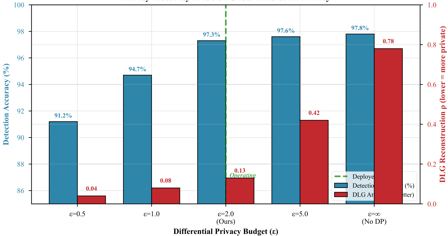
Privacy–Accuracy Trade-off Under Differential Privacy
